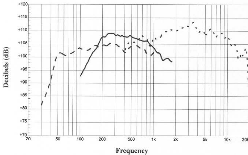
Figure 4—VARIPLEX™-XL Typical Frequency Response of Low / Mid and High Frequency Sections Alone (swept sine-wave input, anechoic environment, (normalized response, from 1 watt, 2 meters from the horn baffle, at 600Hz, with the Microphone axis coincident with the aiming point. (Midway between Mid-Frequency horn and High Frequency horn)
